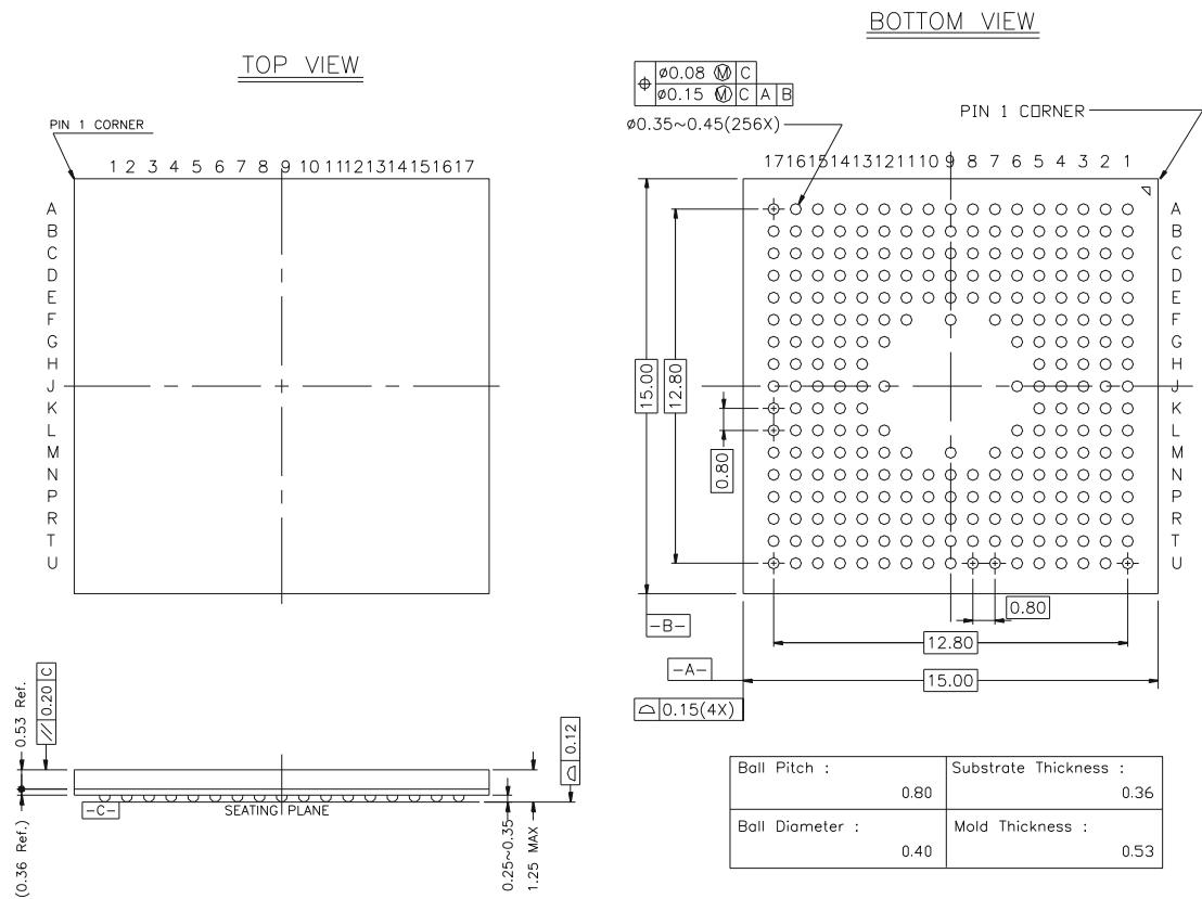
Figure 2. BGA256 (AT91SO100/101)
